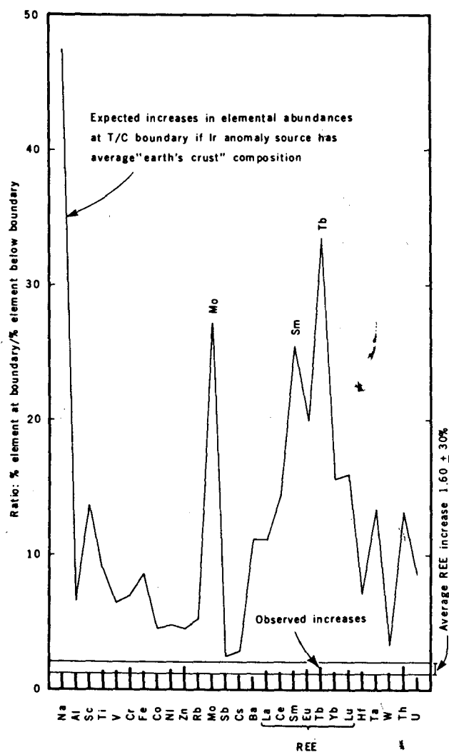
Fig. 10 (left). Comparison of observed elemental abundance patterns in the Gubbio section samples with average patterns expected for crustal material (46). Fig. 11 (right). Comparison of observed elemental abundance patterns in the Gubbio section samples with patterns expected for carbonaceous chondrites (46).
