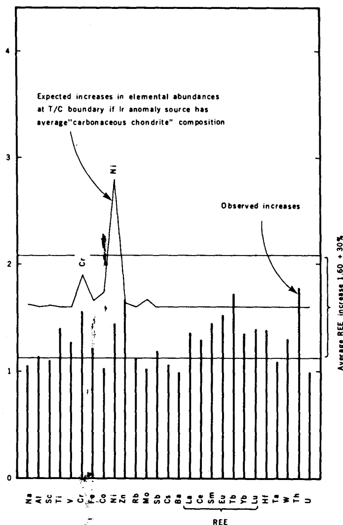
Fig. 10 (left). Comparison of observed elemental abundance patterns in the Gubbio section samples with average patterns expected for crustal material (46). Fig. 11 (right). Comparison of observed elemental abundance patterns in the Gubbio section samples with patterns expected for carbonaceous chondrites (46).
