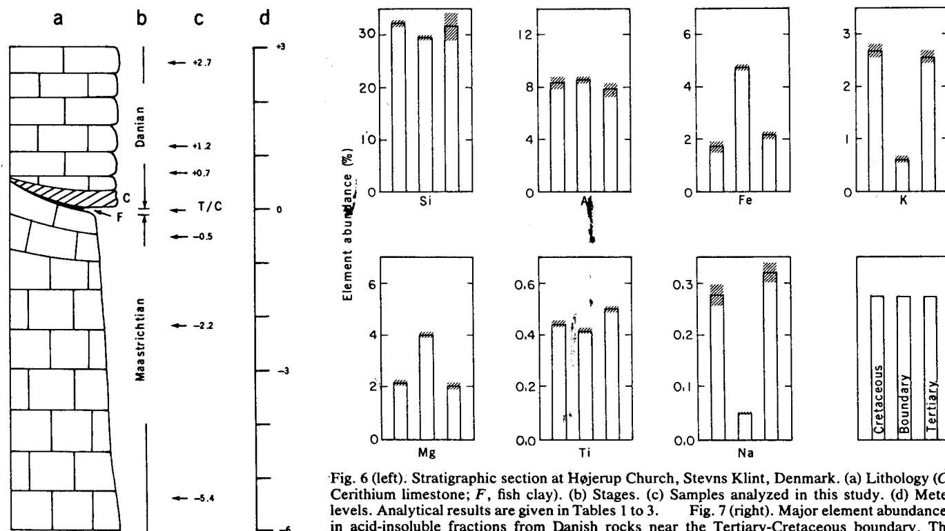
Fig. 6 (left). Stratigraphic section at Højerup Church, Stevns Klint, Denmark. (a) Lithology (C, Cerithium limestone; F, fish clay). (b) Stages. (c) Samples analyzed in this study. (d) Meter levels. Analytical results are given in Tables 1 to 3. Fig. 7 (right). Major element abundances in acid-insoluble fractions from Danish rocks near the Tertiary-Cretaceous boundary. The crosshatched areas for the Cretaceous and Tertiary values each represent root-mean-square deviations for three samples. (Only two measurements of magnesium and silicon were included in the Cretaceous values.) For the boundary layer sample the crosshatched areas are the standard deviations associated with counting errors. Measurements of silicon and magnesium were done by XRF (42), all others were by NAA.
